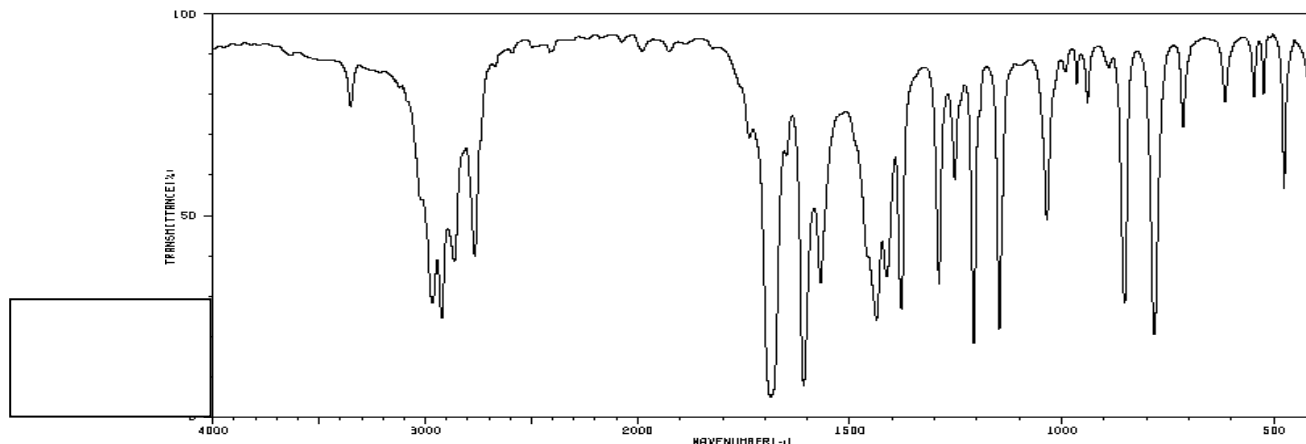
Spectrum 1:
