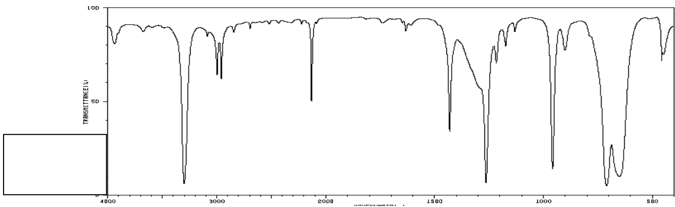
Spectrum 10:
