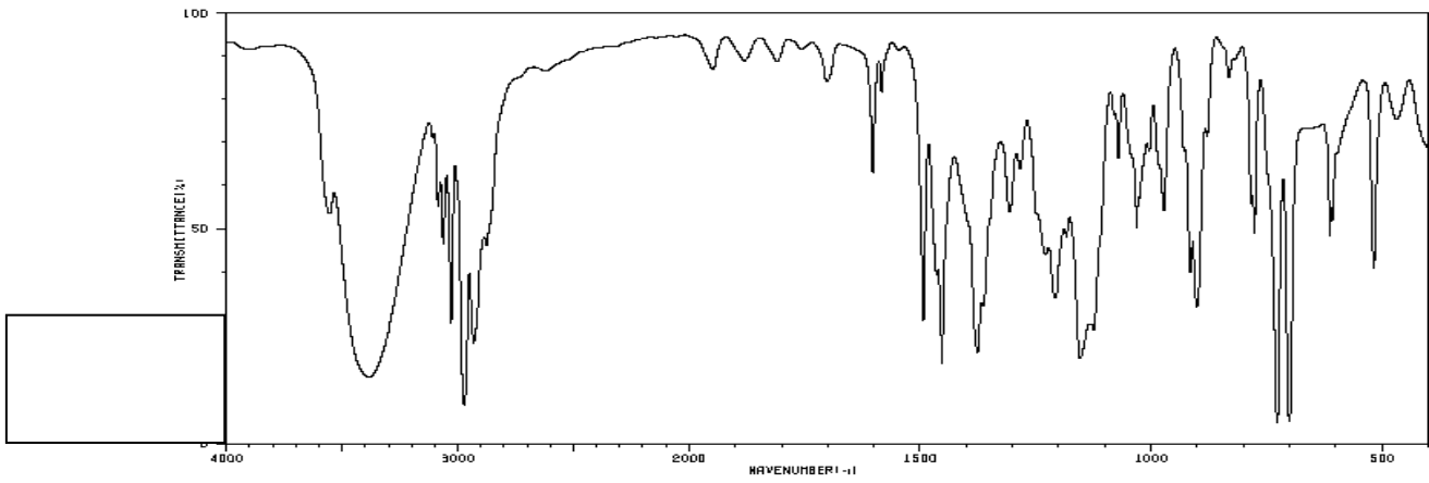
Spectrum 2:
