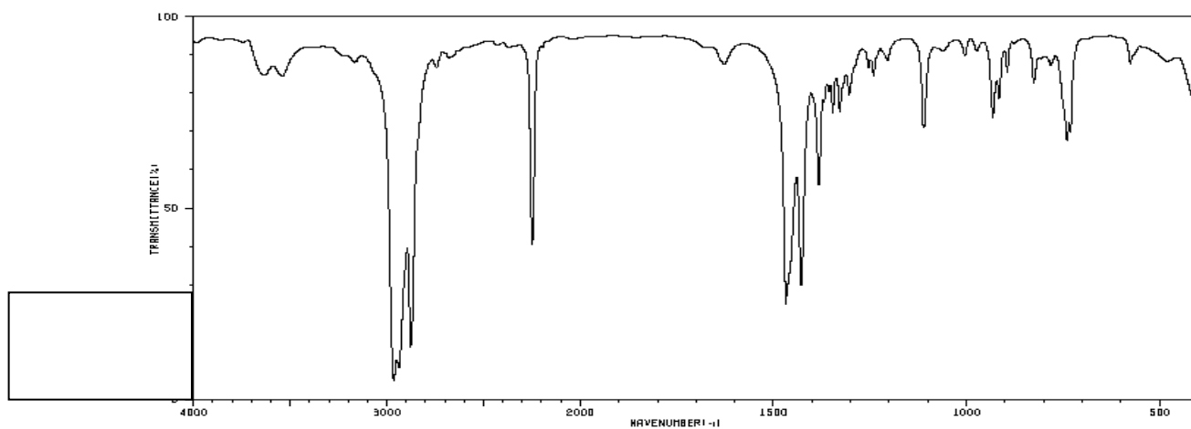
Spectrum 7:
