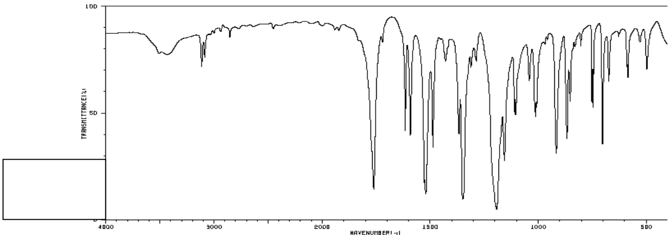
Spectrum 4:
