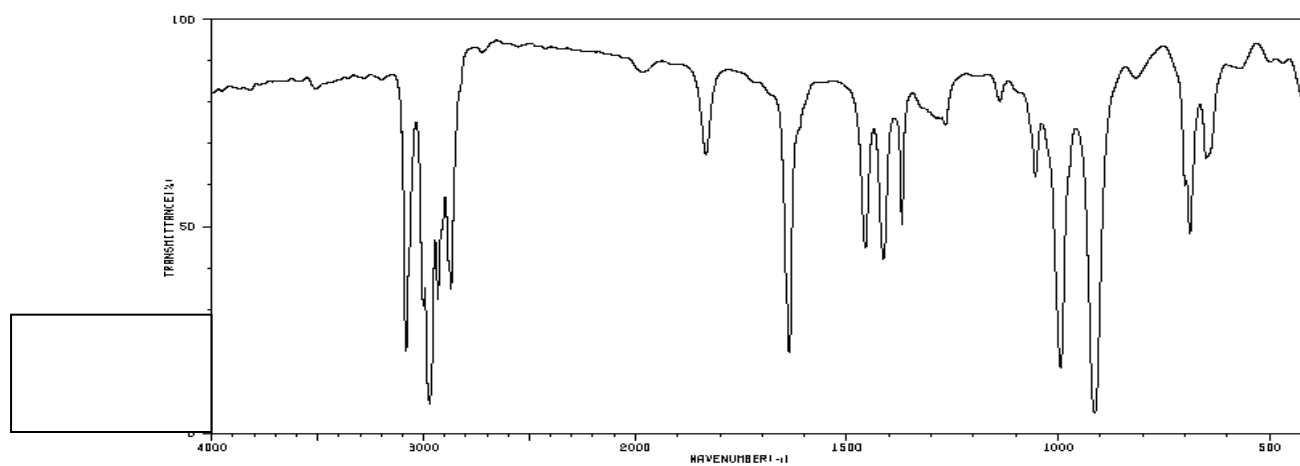
Spectrum 9:
