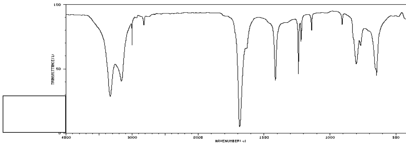
Spectrum 10:
