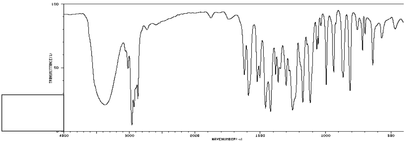
Spectrum 3:
