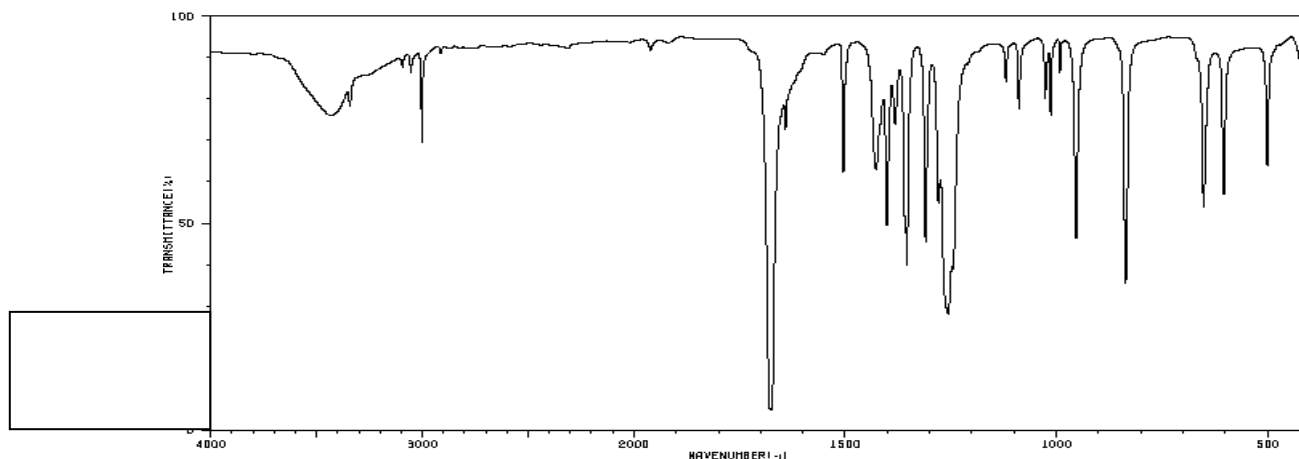
Spectrum 1:
