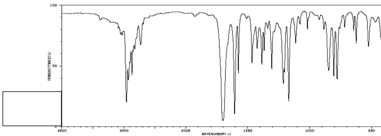
Spectrum 6:
