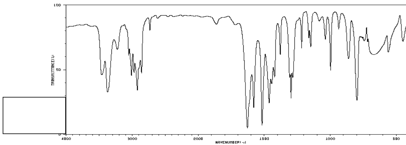
Spectrum 8:
