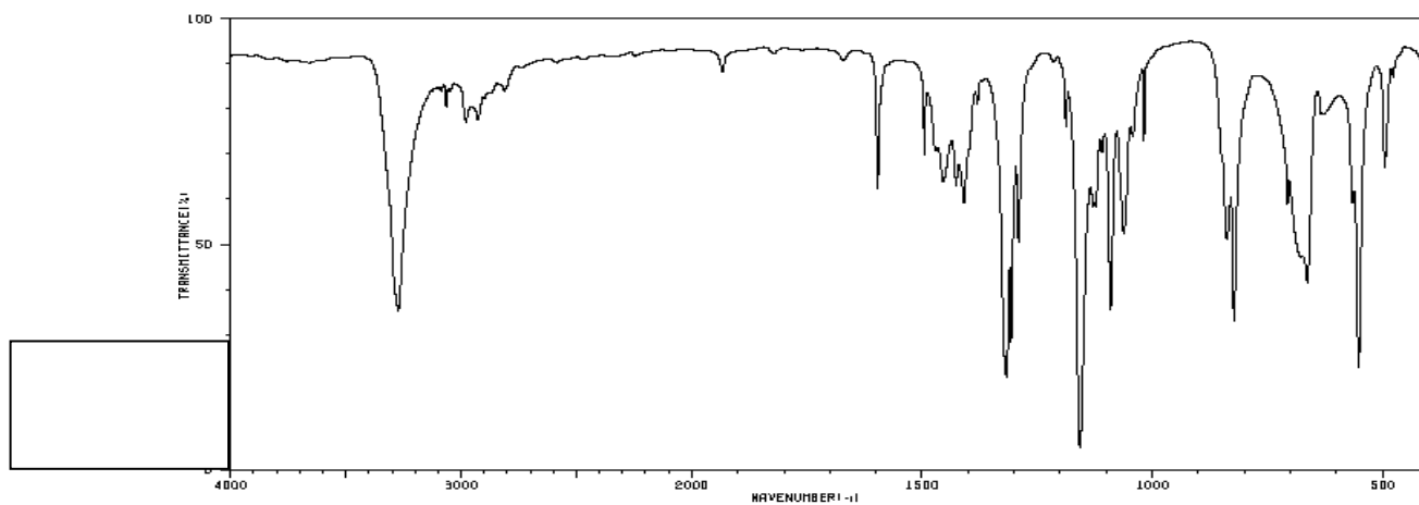
Spectrum 6:
