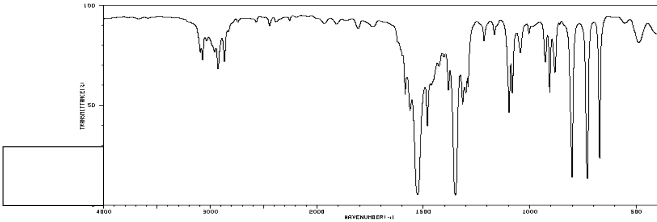
Spectrum 10:
