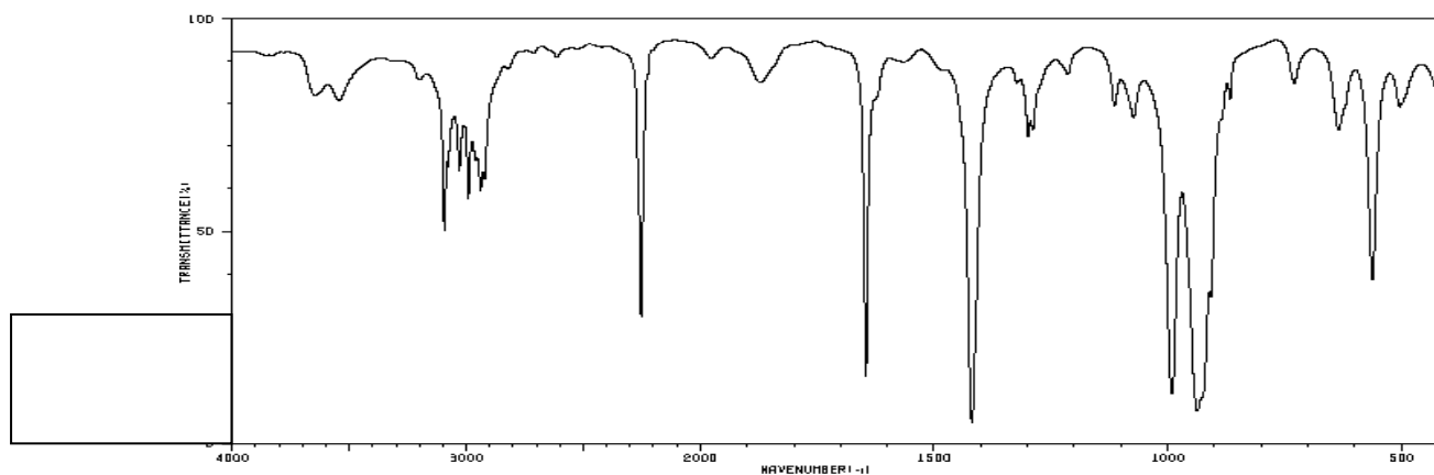
Spectrum 6:
