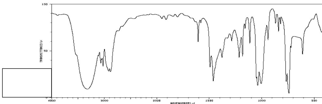
Spectrum 1:
