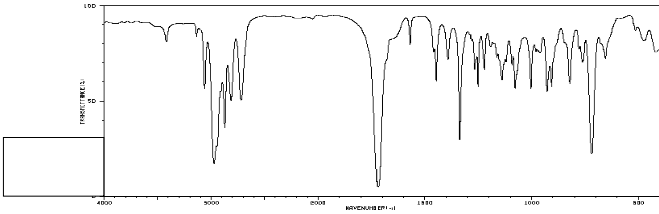
Spectrum 2:
