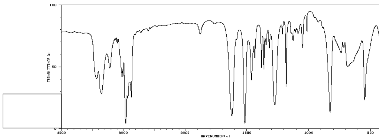
Spectrum 7:
