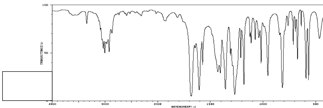
Spectrum 6:
