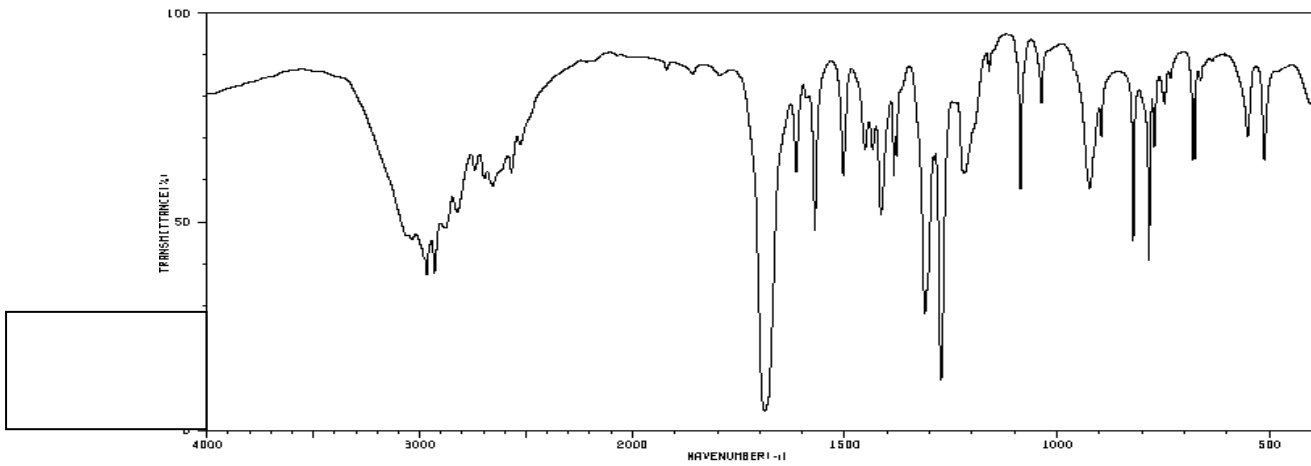
Spectrum 9:
