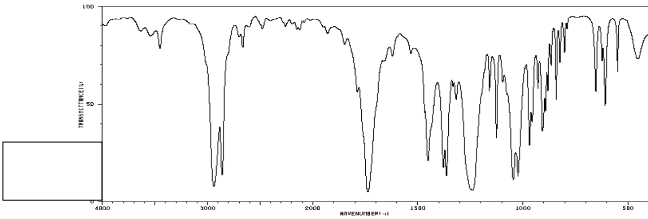
Spectrum 3:
