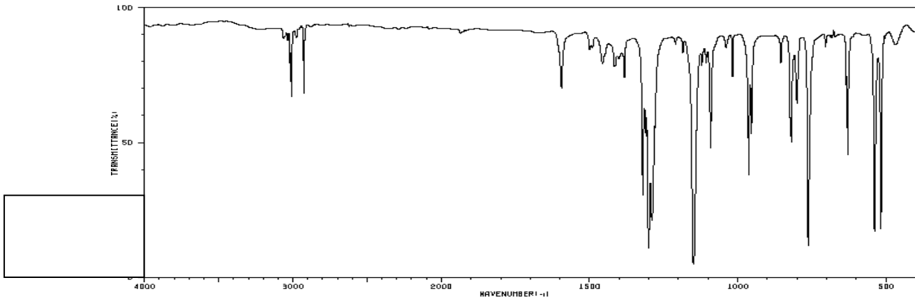
Spectrum 8:
