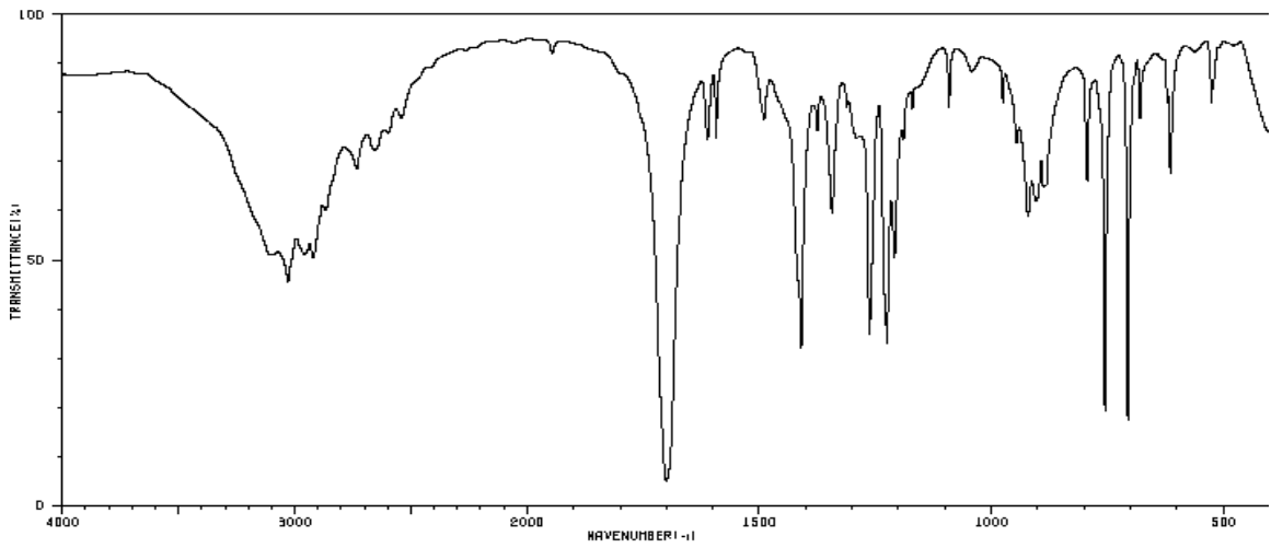
Spectrum 4:
