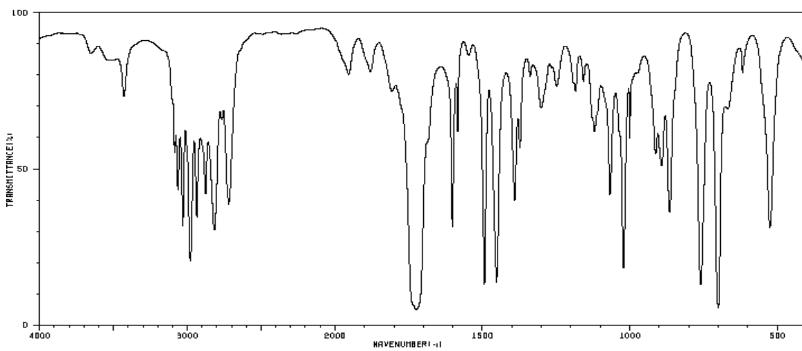
Spectrum 5:
