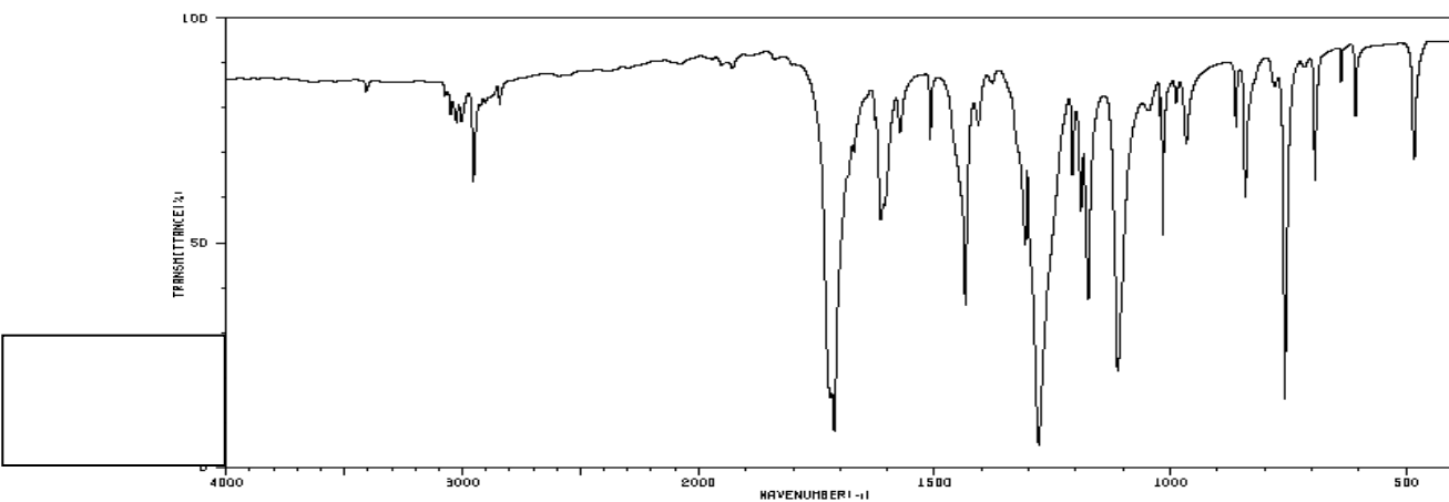
Spectrum 4:
