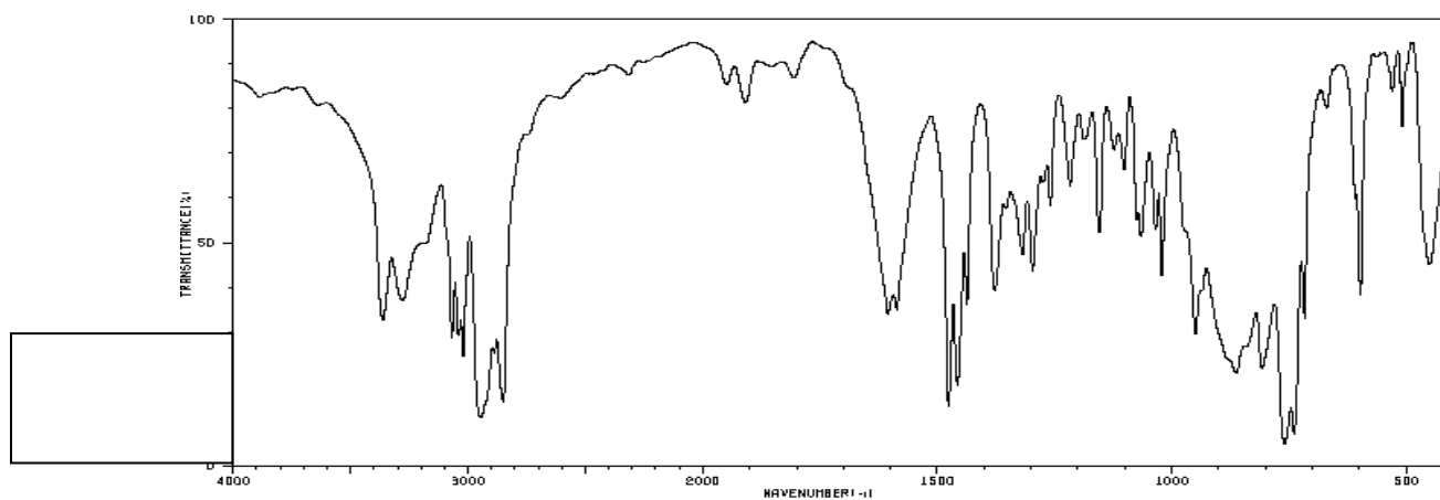
Spectrum 6:
