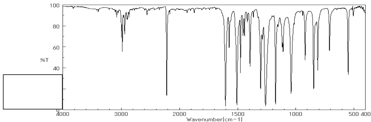
Spectrum 1:
