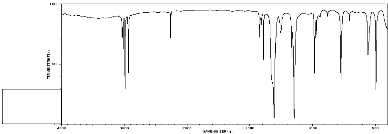
Spectrum 10:
