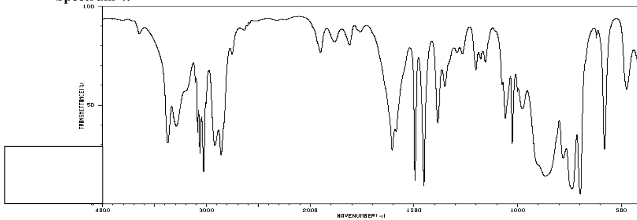
Spectrum 4:
