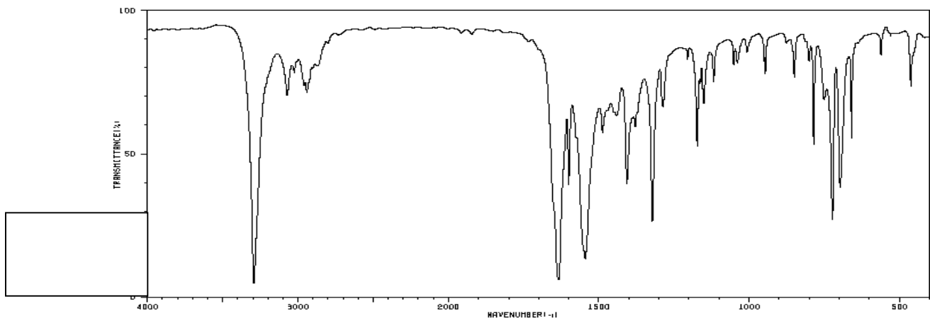
Spectrum 9:
