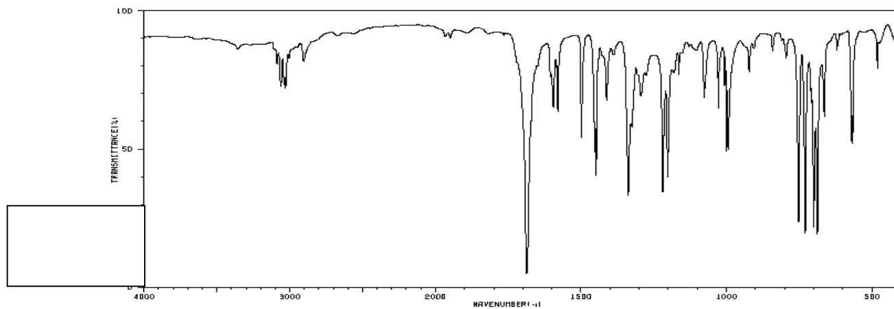
Spectrum 2:
