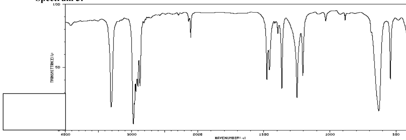
Spectrum 3:
