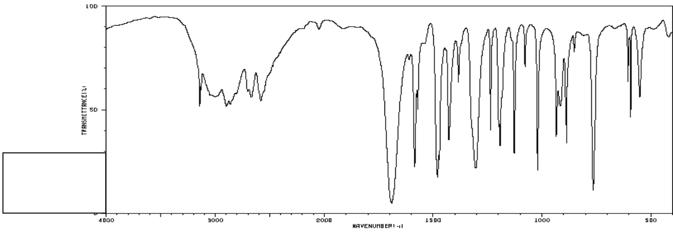
Spectrum 5:
