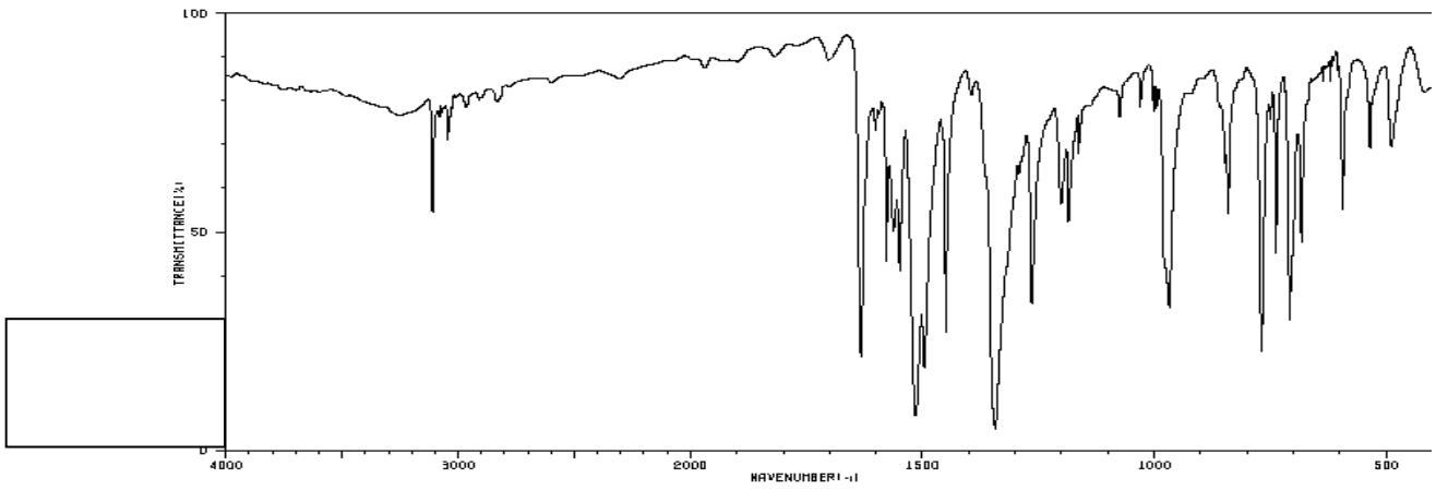
Spectrum 3:
