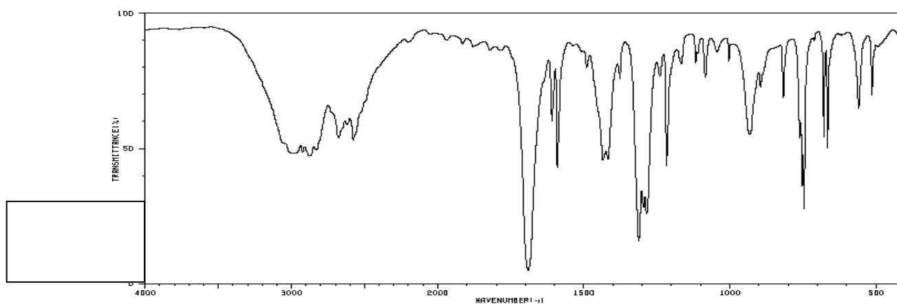
Spectrum 5:
