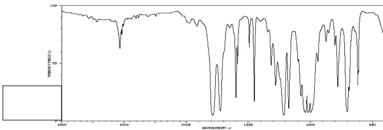
Spectrum 9:
