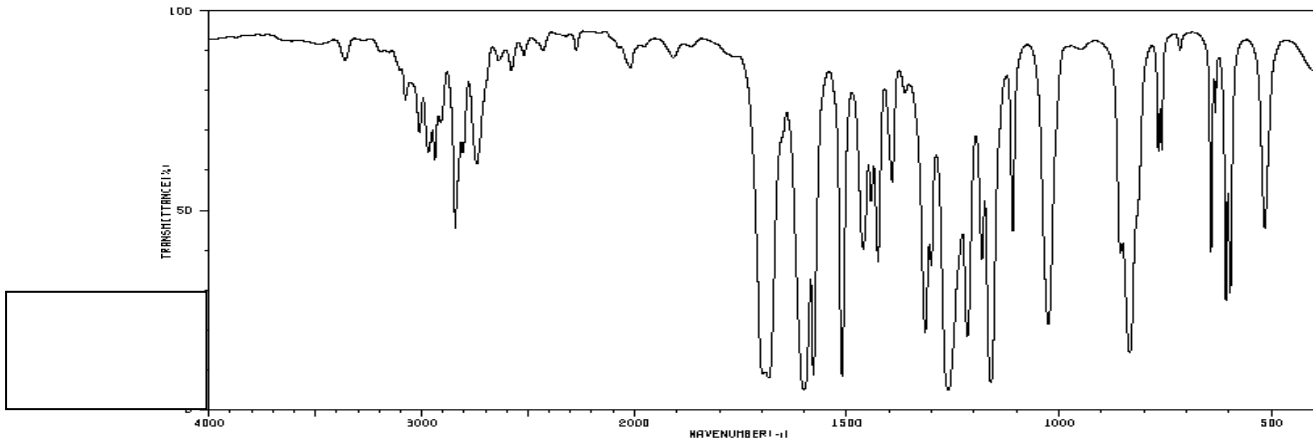
Spectrum 2:
