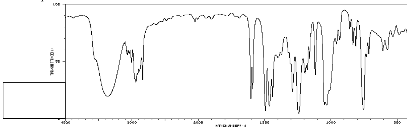
Spectrum 1:
