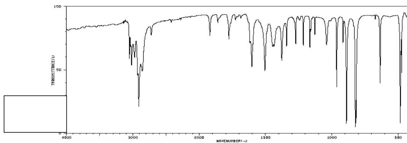
Spectrum 7:
