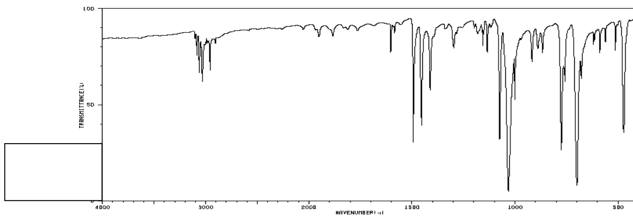
Spectrum 6:
