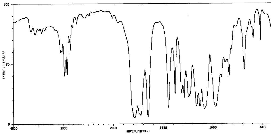
Spectrum 10:
