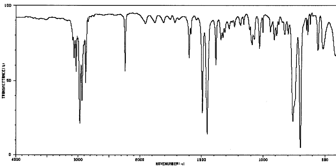
Spectrum 6:
