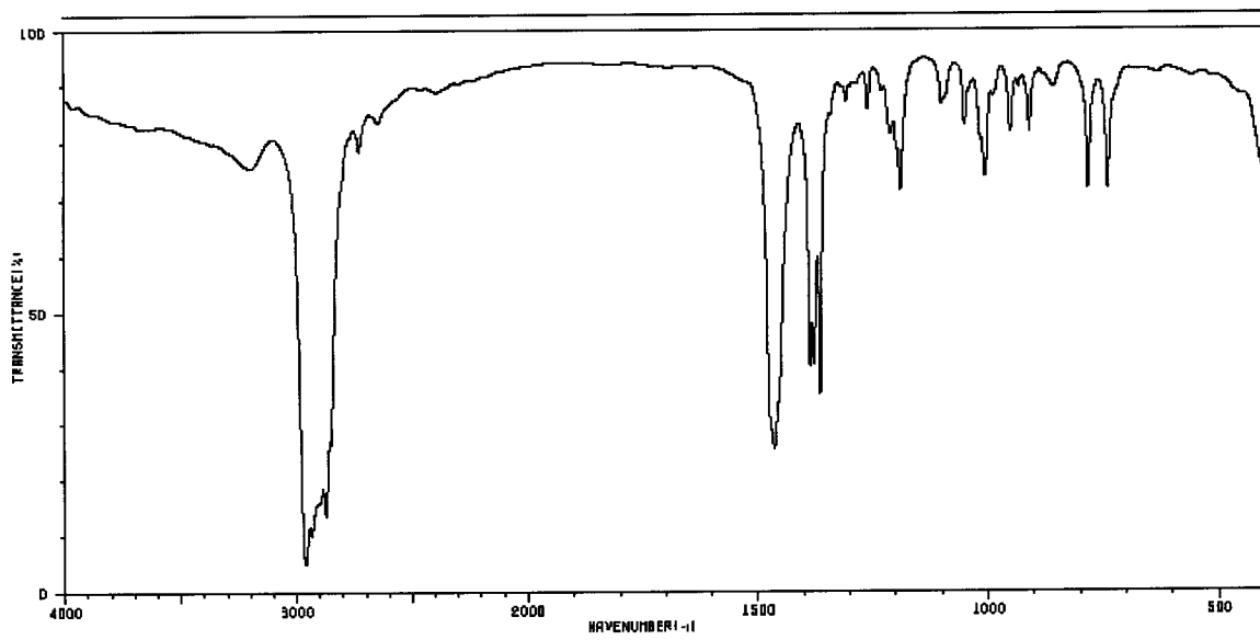
Spectrum 9:
