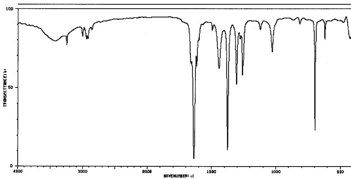
Spectrum 3:
