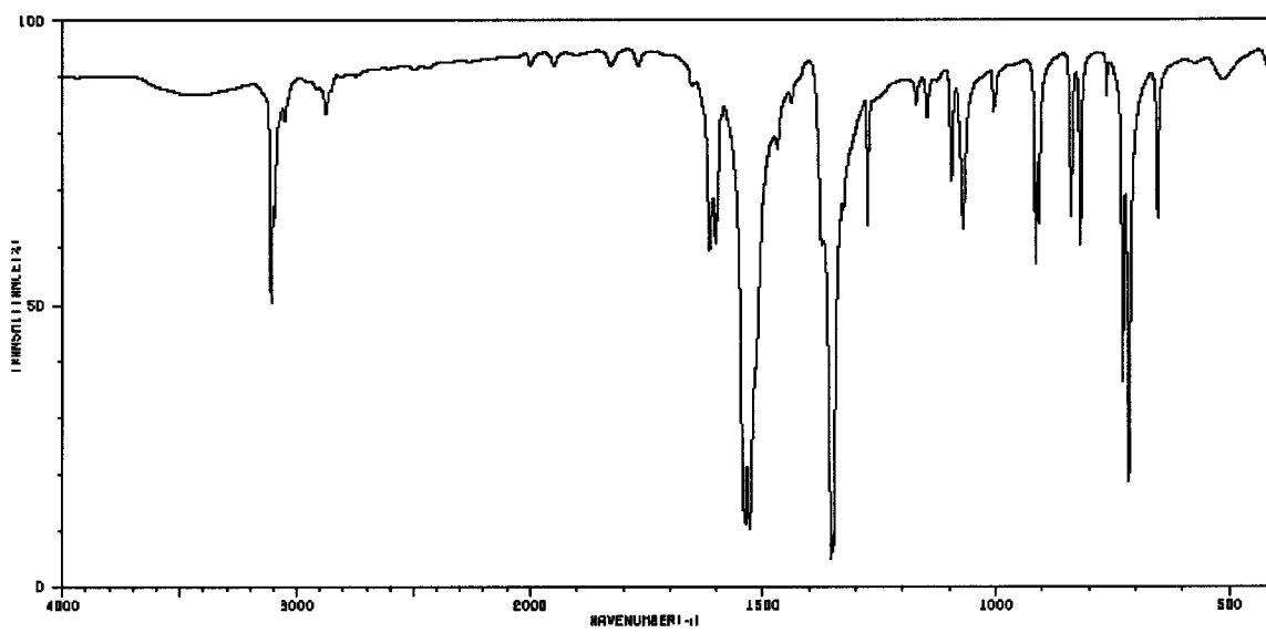
Spectrum 8:
