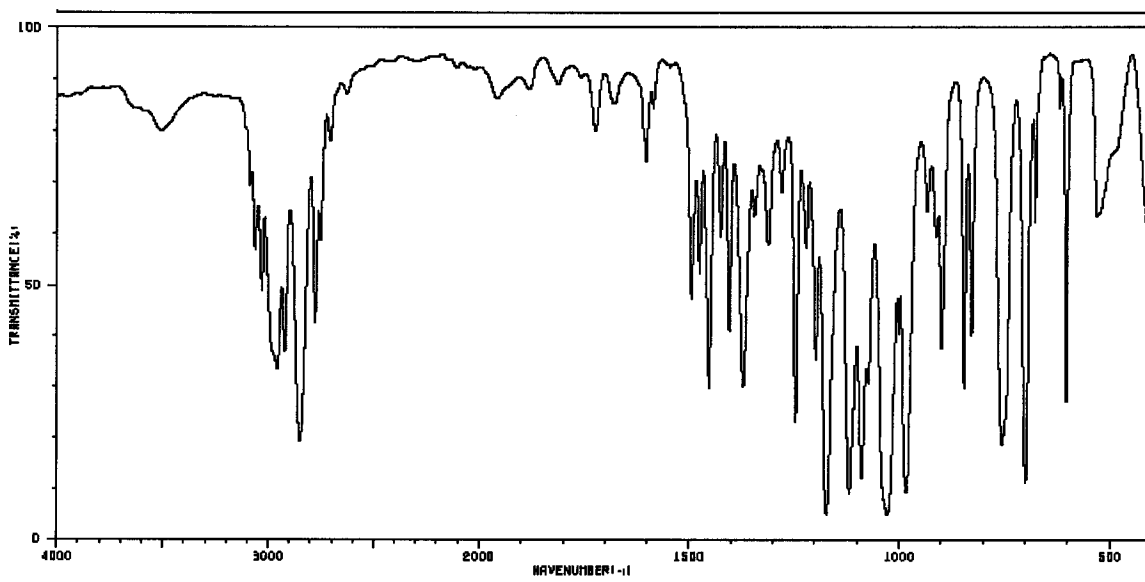
Spectrum 4:
