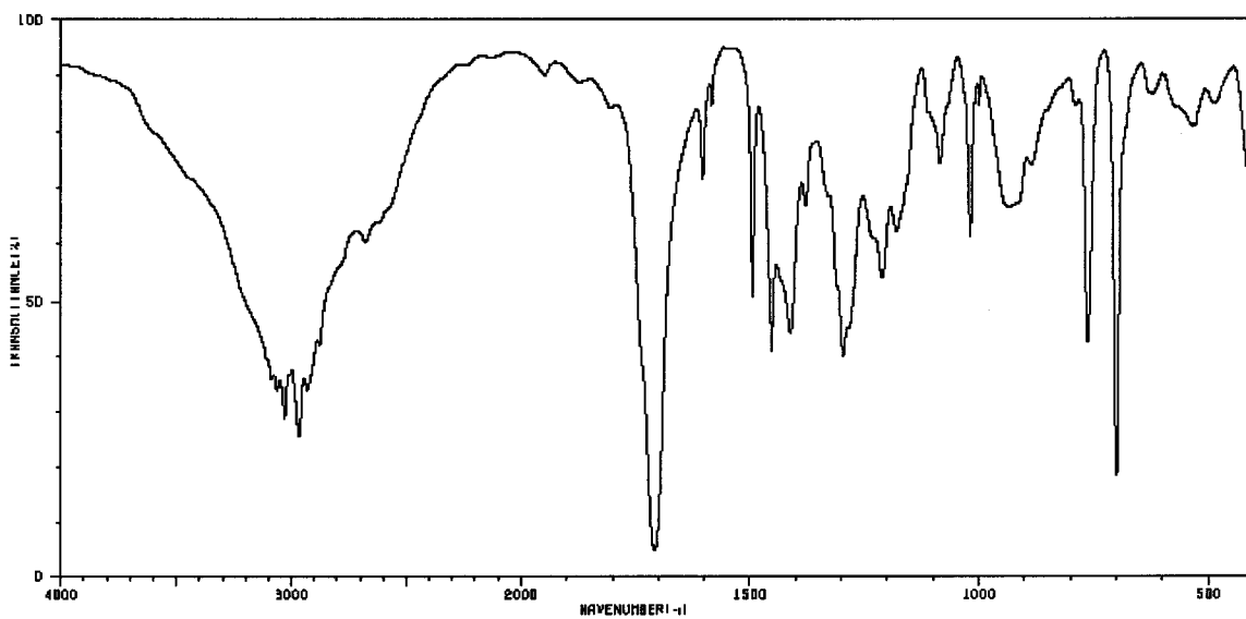
Spectrum 2:
