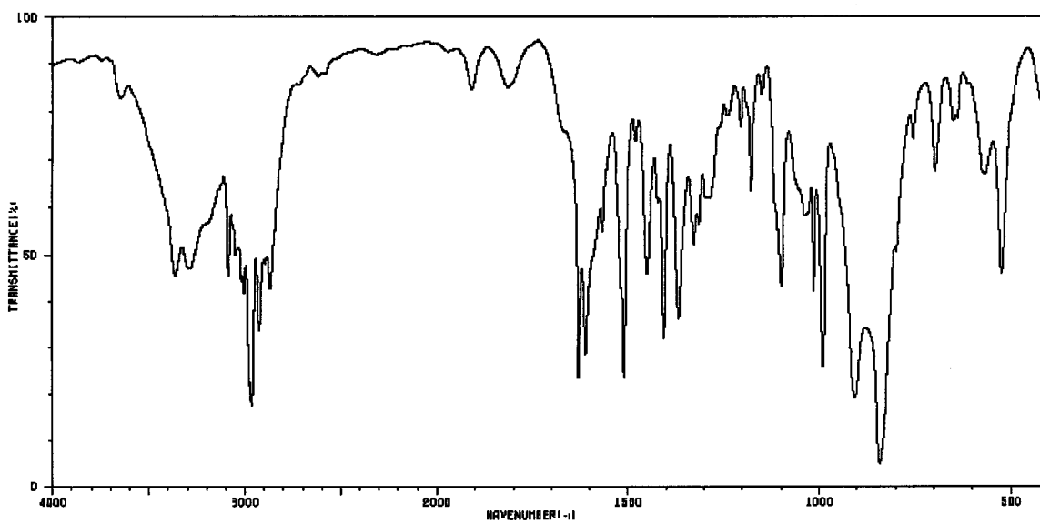
Spectrum 7:
