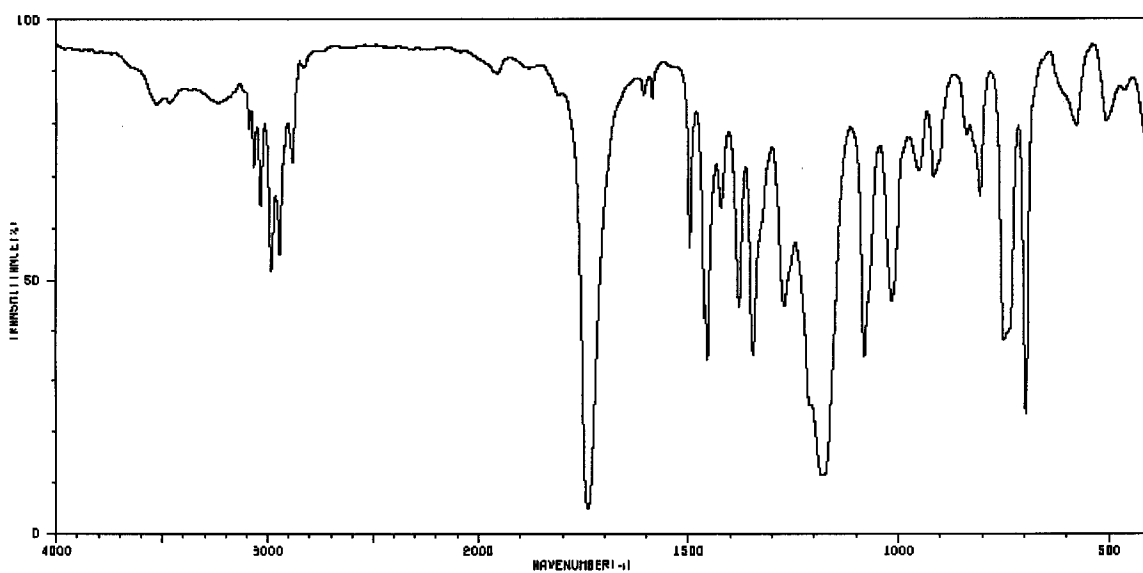
Spectrum 1:
