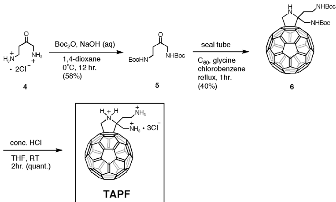
Scheme II. Synthesis of TAPF.
