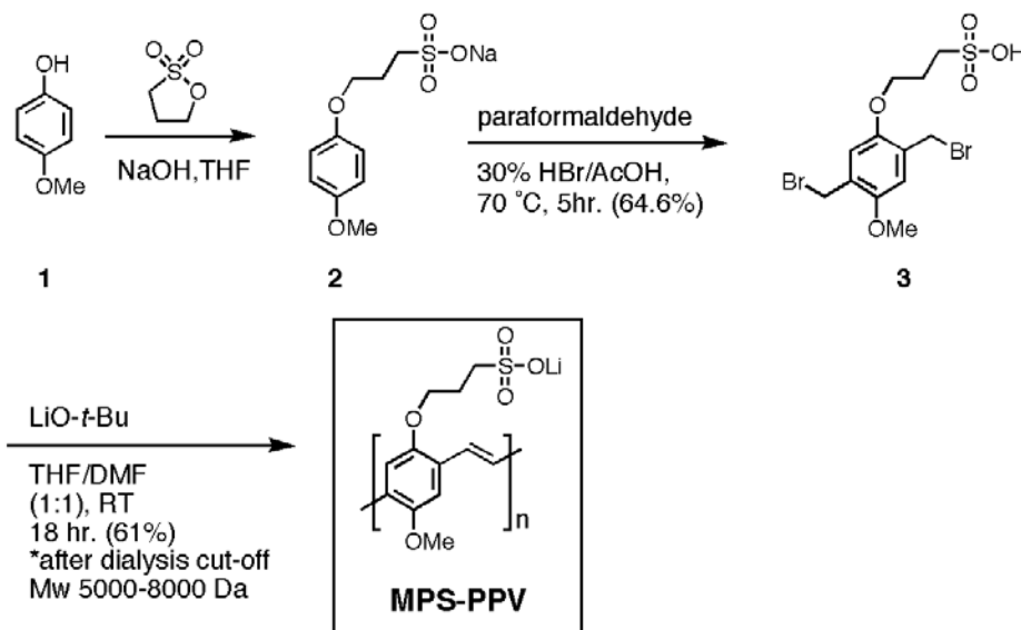
Scheme I. Synthesis of MPS-PPV.
